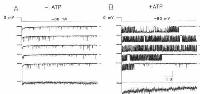
FIGURE 5 Desensitization of the native Ca release channel. The records were taken from the same channel at 100 \mu M free Ca (A) and after addition of 2 mM ATP to the myoplasmic solution (B) (bilayer 94207). The bottom traces were ensemble averages of five complete experiments. The solid line is the best fit exponential decay function, y = -5.63 \times \exp(-t/4.94(s)) - 5.38 (pA). The vertical bar corresponds to a 30 pA current for the single channel traces, and 6 pA for the ensemble averages.
