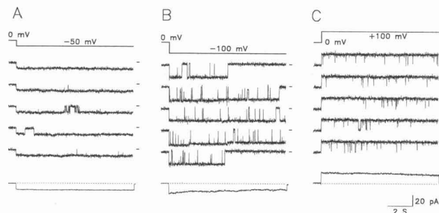
FIGURE 2 Voltage-dependent inactivation of the ryanodine-activated channel. Selected consecutive single channel records through a ryanodine-activated channel with test pulses to -50 mV (A), -100 mV (B), and +100 mV (C) (bilayer 93N23). The corresponding ensemble averages at different voltages are shown in the bottom traces. Marks at the right of each trace correspond to the baseline current.
